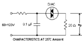
* CIRCUIT FOR PEAK OUTPUT VOLTAGE TEST
