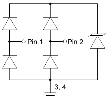
2-Line Protection
