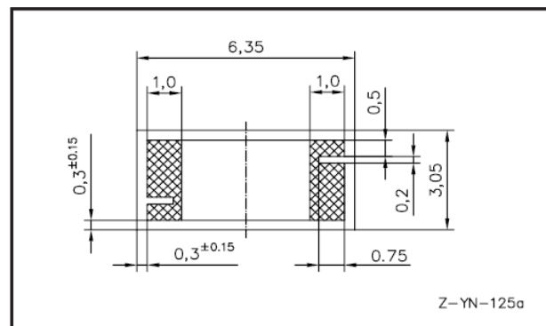
Layout Typ A / Layout type A
