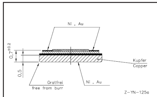
Layout Typ A / Layout type A
