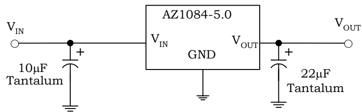
Figure 12. Typical Applications of AZ1084
