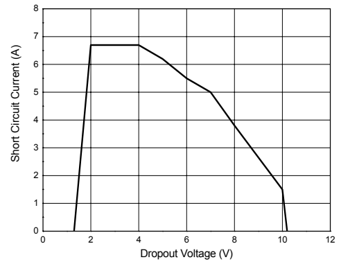
Figure 9. Short Circuit Current vs. Dropout Voltage
