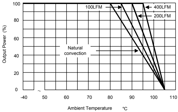
Derating Curve (5V&12Vin)
