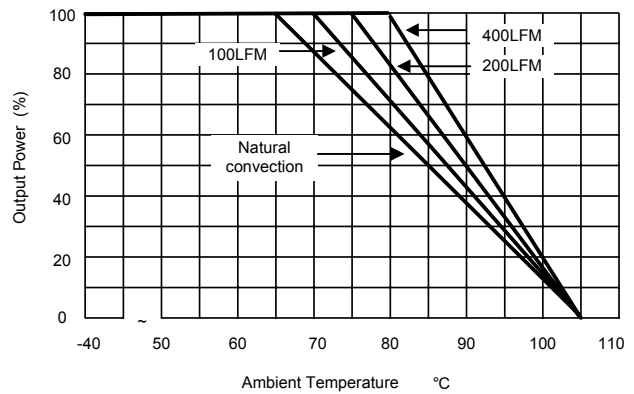
Derating Curve (24Vin)
