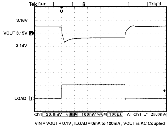
Load Transient
