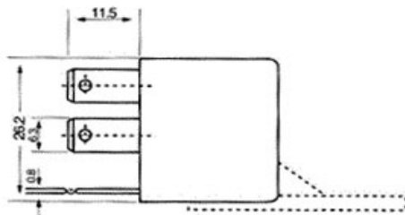
1 Form A
