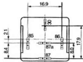
1 Form C
