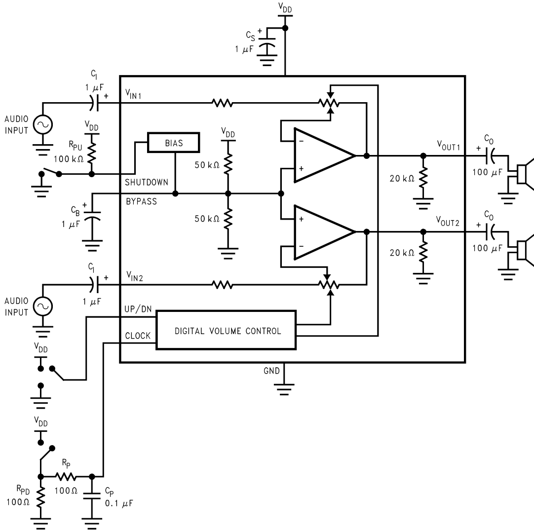
FIGURE 3. Demoboard Schematic
