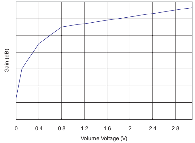
15. Gain vs DC voltage
