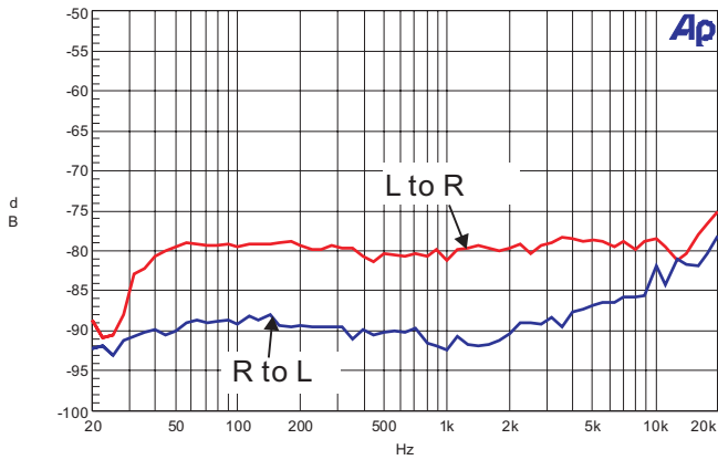
8. Crosstalk
