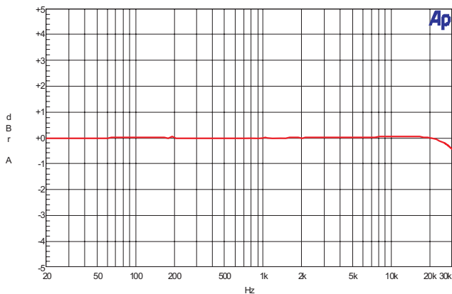
9. Frequency Response ( V_o=1.0V_{rms} )
