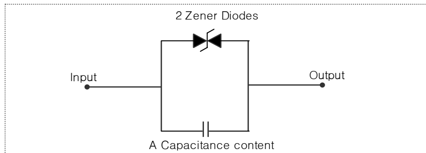
Fig.2 Equivalent Circuit
