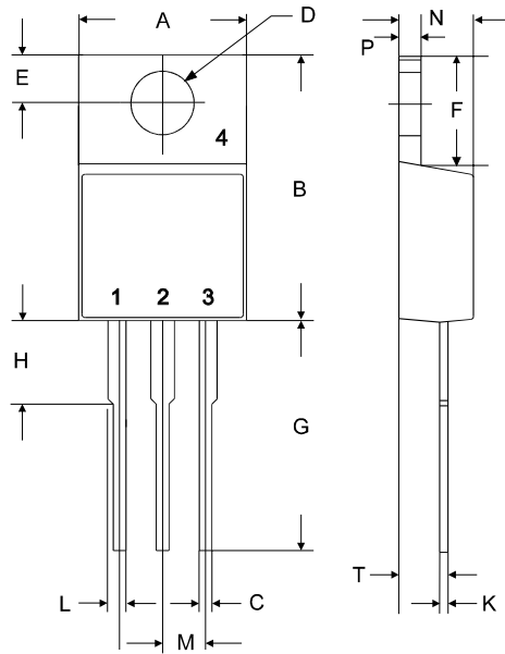
PG-TO220-3-1
