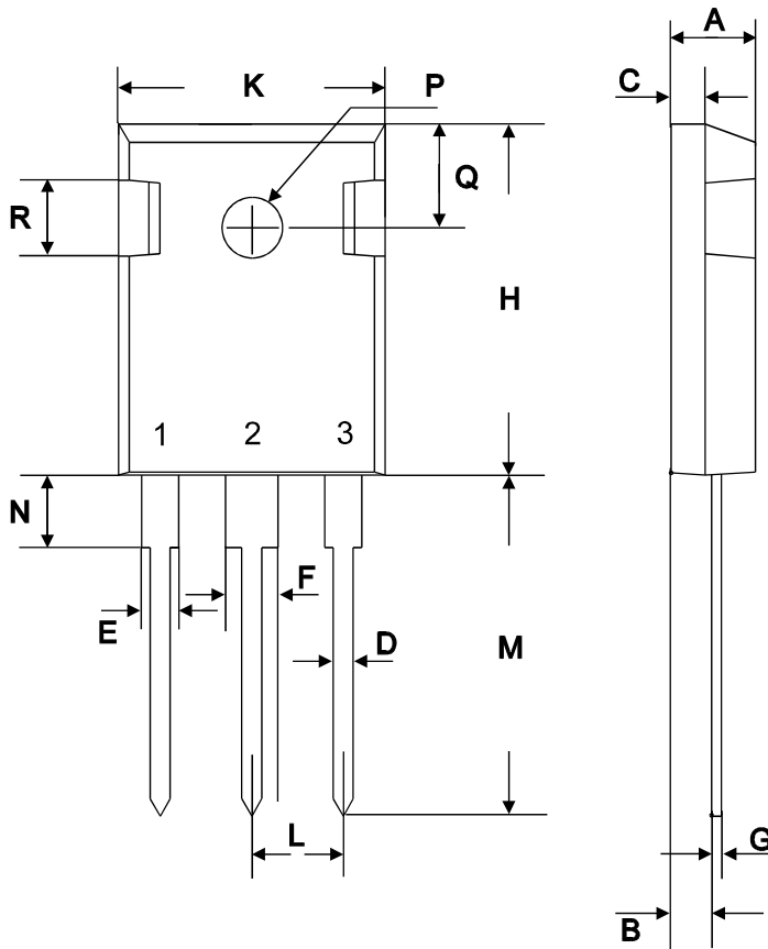
PG-TO247-3-1
