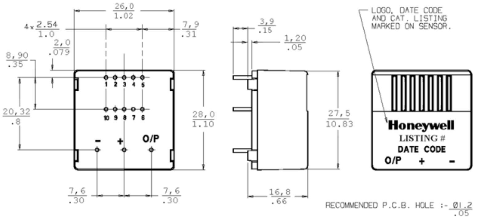
Mounting Dimensions - for reference only (mm/in)
