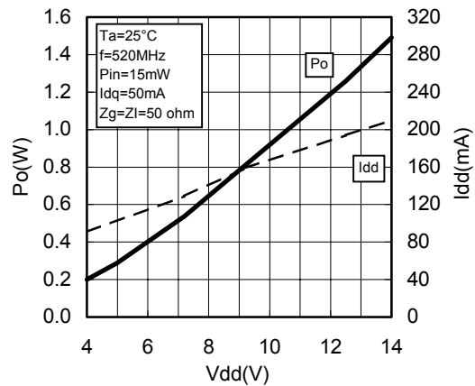
Vdd-Po CHARACTERISTICS
