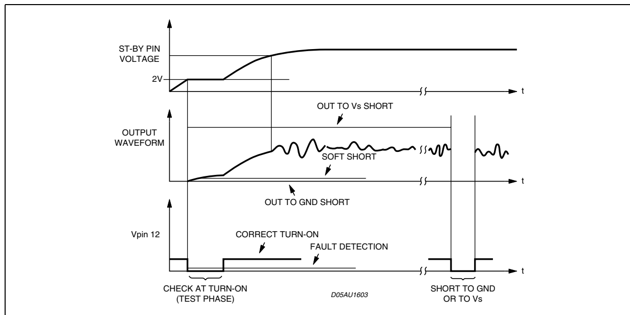
Figure 34. Fault Waveforms
