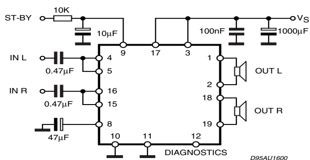
Figure 11. Double Bridge
