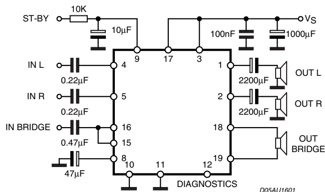
Figure 12. Stereo Bridge
