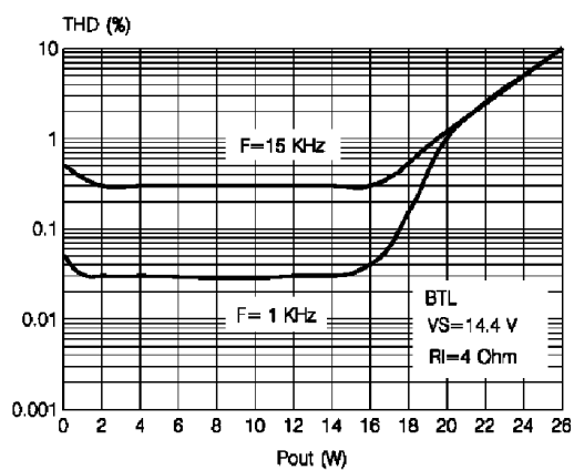
Figure 20. Distortion vs. Output Power
