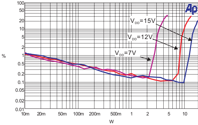
1. THD vs. Power
