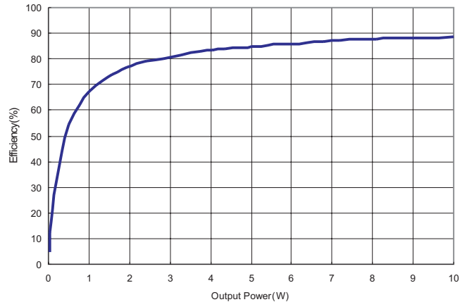
12. Efficiency vs Power
