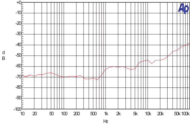
7. Power Supply Ripple Rejection
