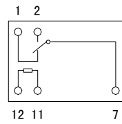
FormC
