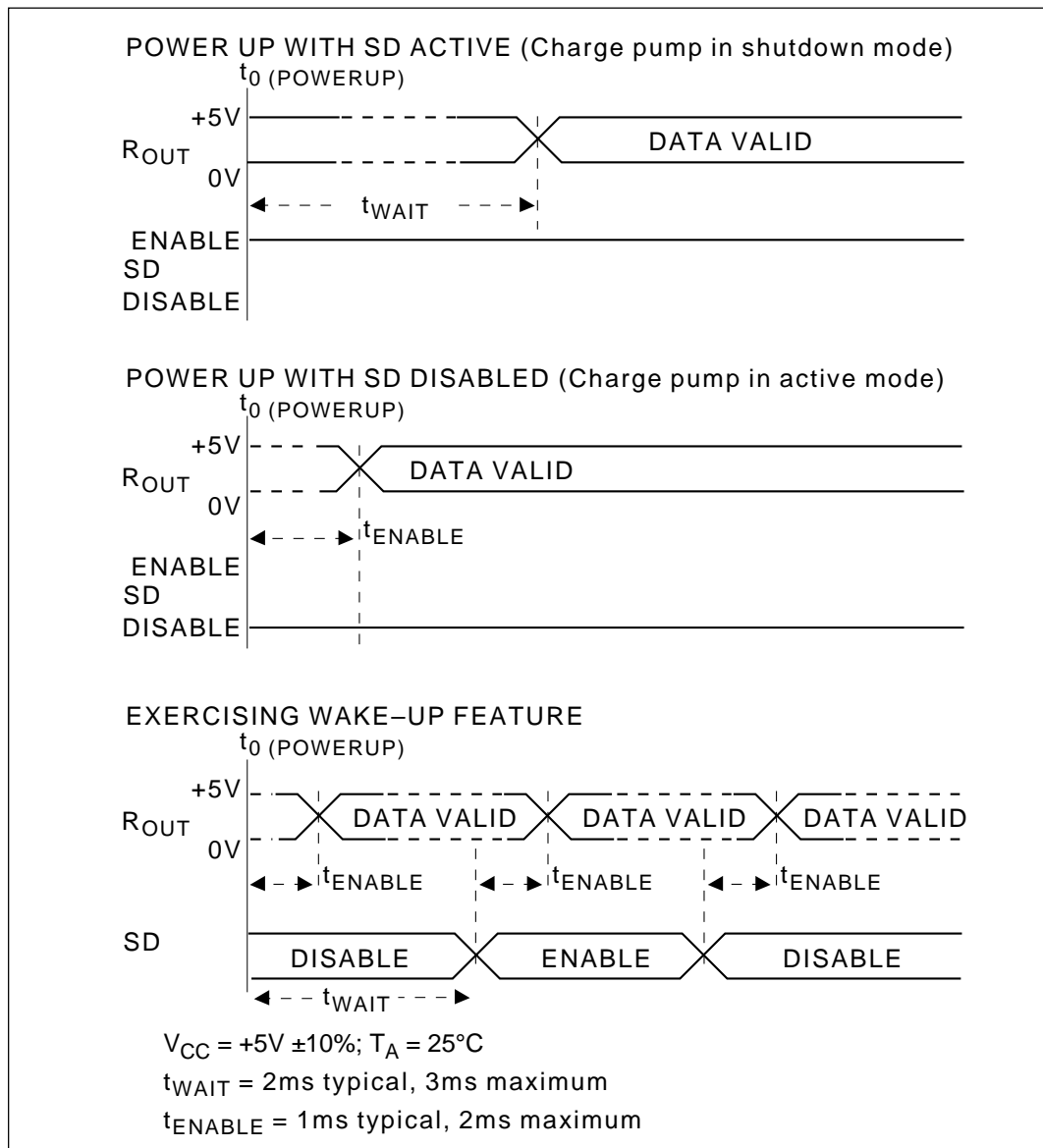
Figure 6. Wake-Up Timing
