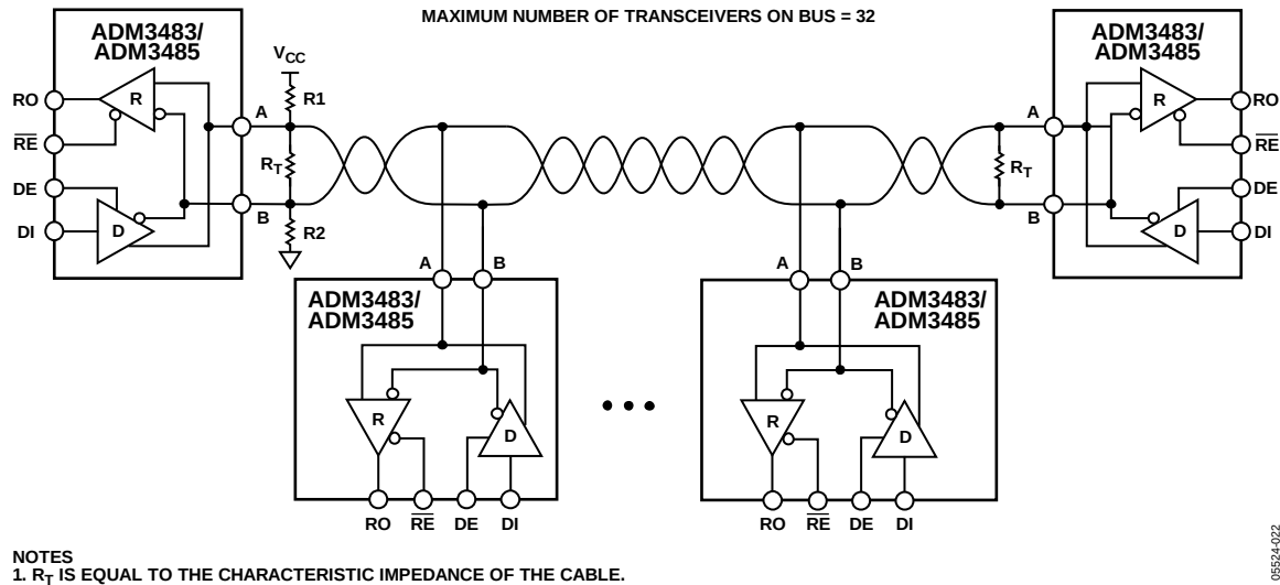
Figure 32. ADM3483/ADM3485 Typical Half-Duplex RS-485 Network
