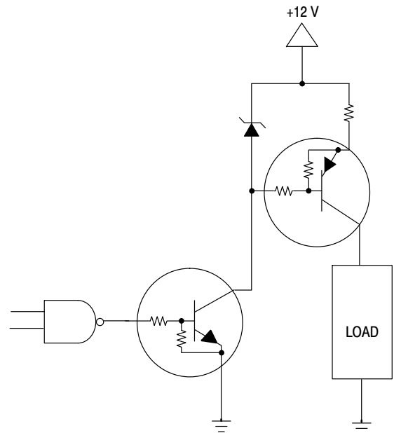
Figure 35. Inexpensive, Unregulated Current Source
