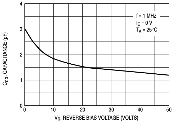
Figure 15. Output Capacitance
