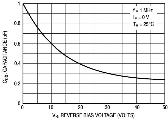
Figure 20. Output Capacitance
