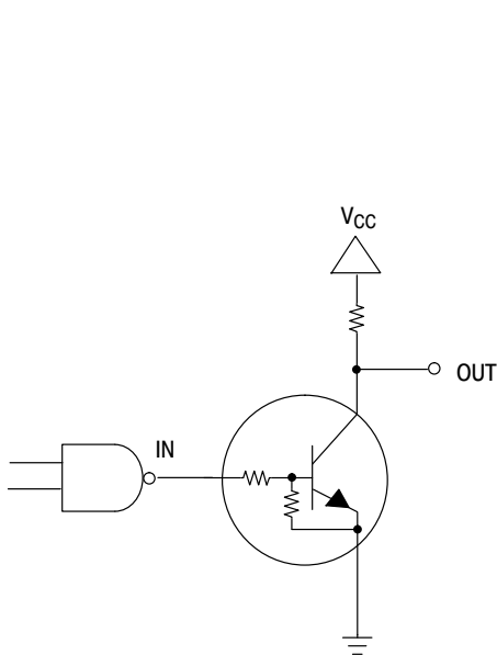
Figure 34. Open Collector Inverter: Inverts the Input Signal
