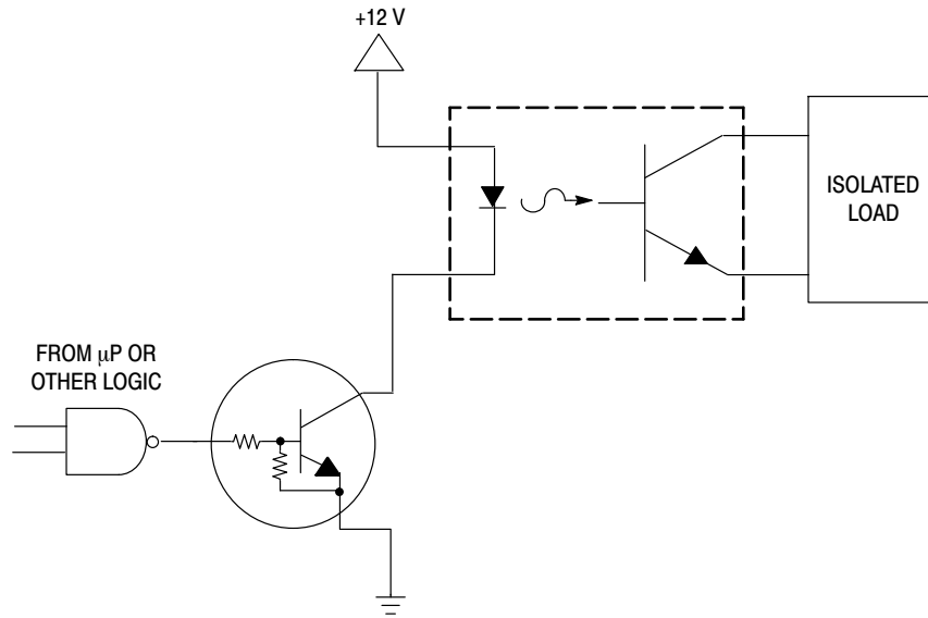
Figure 33. Level Shifter: Connects 12 or 24 Volt Circuits to Logic
