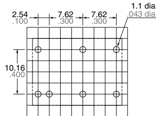
<2 Form A> Single side stable (Deenergized condition) 2 coil latching (Reset condition)
