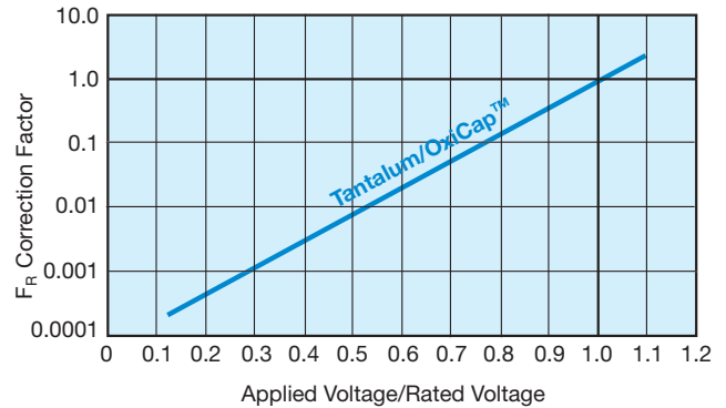
Figure 2a. Correction factor to failure rate F_R for voltage derating of a typical component (60% con. level).
