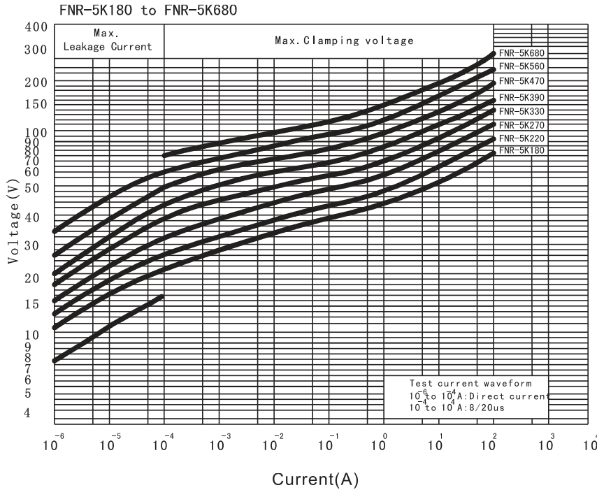
V-I Curve
