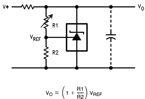
Shunt Regulator
