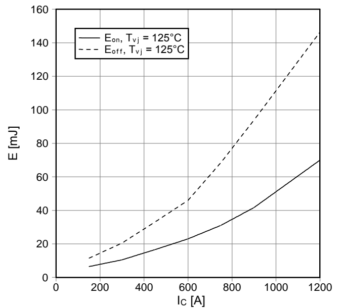
Schaltverluste IGBT-Wechselr. (typisch) switching losses IGBT-inverter (typical) E_{on} = f(I_c) , E_{off} = f(I_c) V_{GE} = \pm 15\text{ V} , R_{Gon} = 1,5\ \Omega , R_{Goff} = 1,5\ \Omega , V_{CE} = 600\text{ V}
