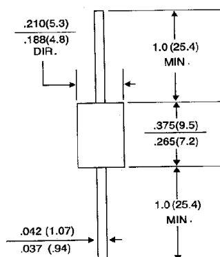
DO-201AE
