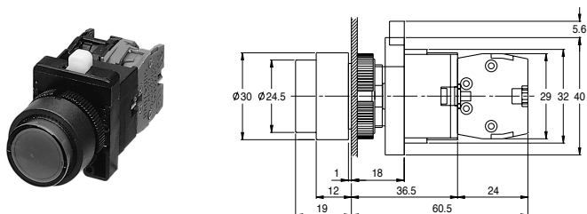
ARX-P (Direct supply /Momentary)
