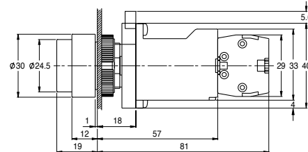
ARX-S (Direct supply /Momentary)
