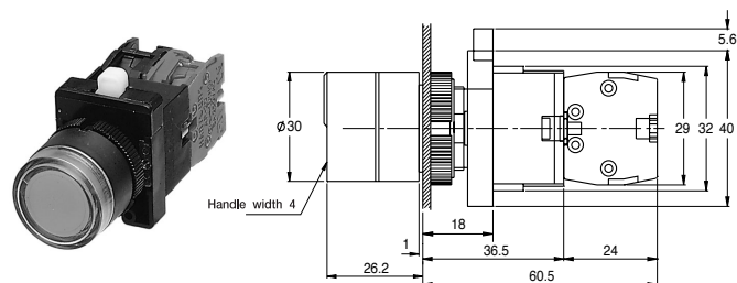
ARX-G (Direct supply /Momentary)
