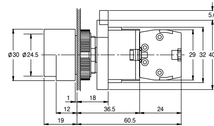
ARX-H (Direct supply /Momentary)
