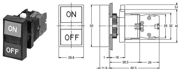
ARX-S (Direct supply /Momentary)
