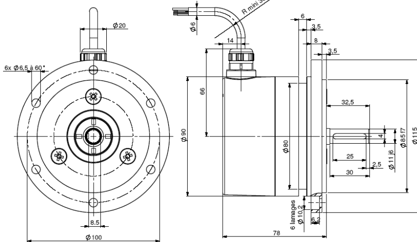
PIF_12 connection G6R (radial M23)
