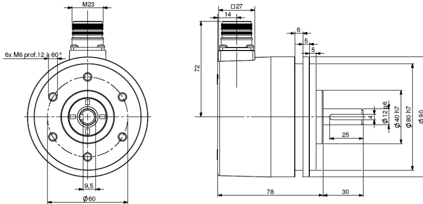
PIF_12 connection G6R (radial M23)
