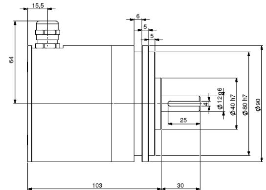
PIF_12 connection BR (terminal box)
