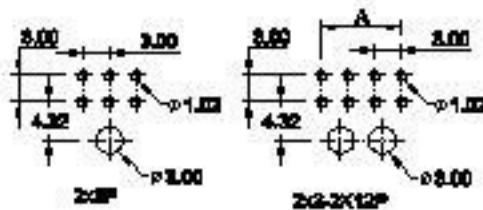
PCB LAYOUT PATTERN DIM(REF)
