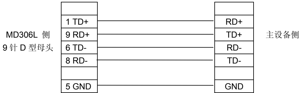
MD2-FREEPTC-RS422 连线图
