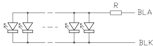
Backlight Circuit Scale=free
