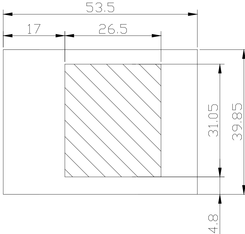
Figure 3: Component (Bottom) View
