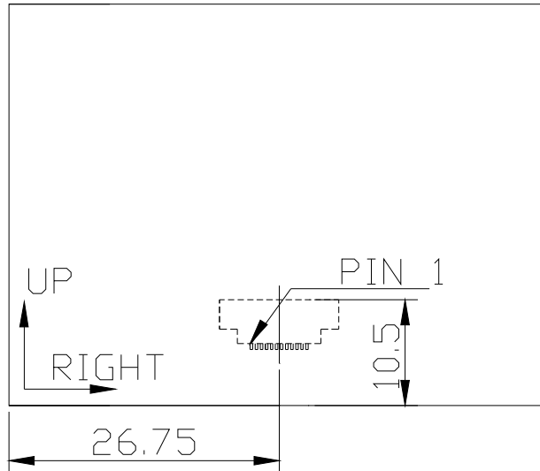
Figure 6: TOP View
