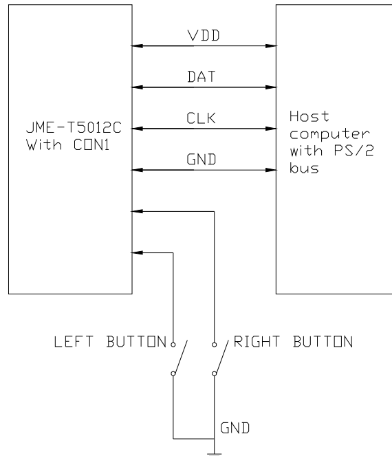
Figure 7: Touchpad/Host Connection (PS/2)
