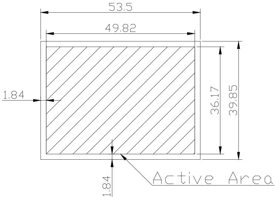
Figure 1: Sensor (Top) View
