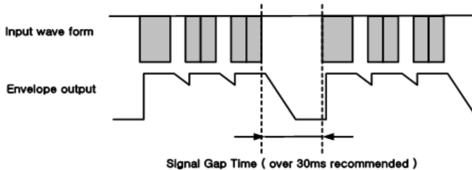
Figure 2 Recommended repeated code format
