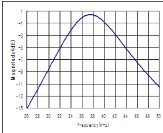
Typical Band-pass Curve
