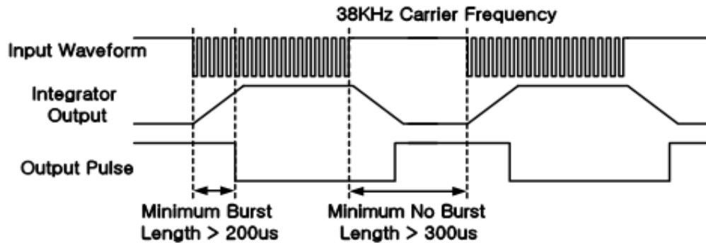
Figure 1 Minimum burst length & No burst length
