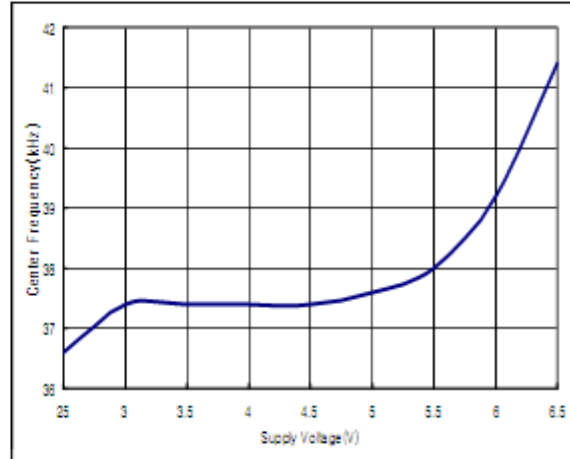
Center Frequency vs supply voltage
