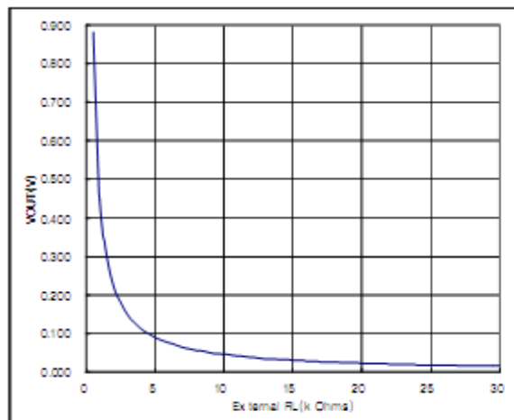
V_{OL} vs Pull-up resistance
