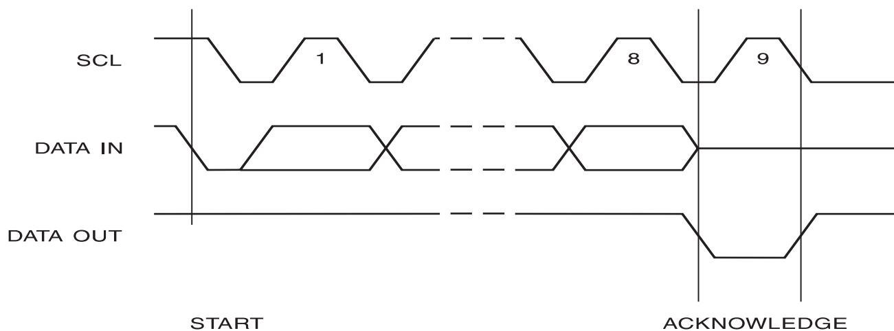
Figure 6. Output Acknowledge
