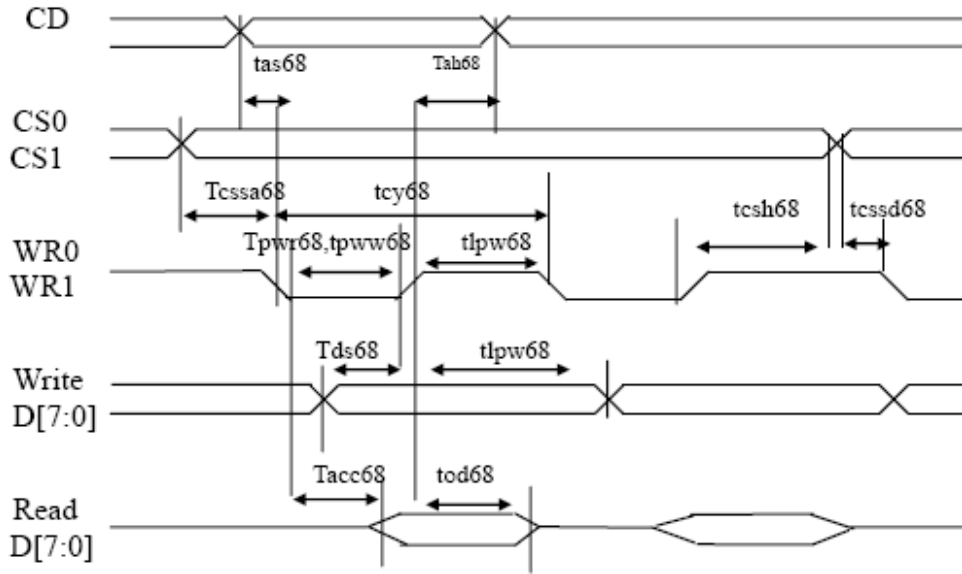
Parallel Bus Timing Characteristics (for 8080 MCU)
