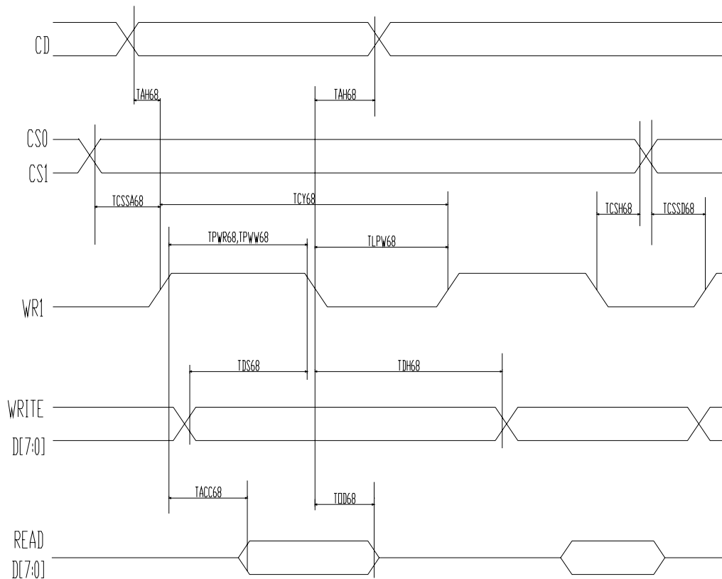
Parallel Bus Timing Characteristics (for 6800 MCU)
