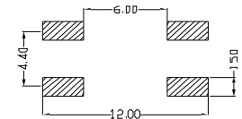
SMD SOLDERING PAD
