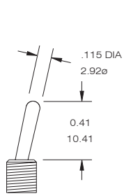
S (STD)
