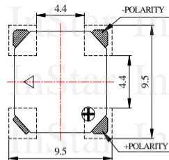
PCB Pad Size
