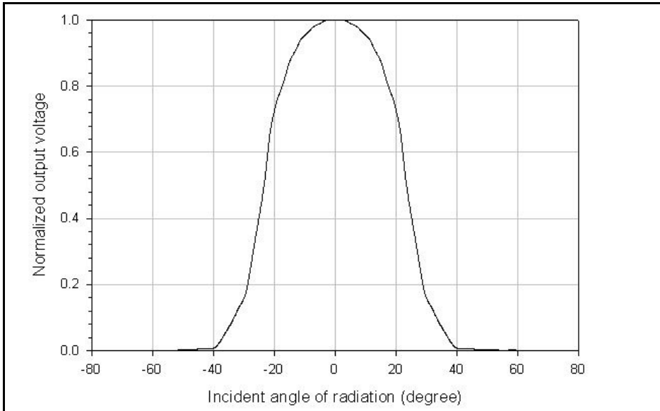
Figure 3: Field of view curve
