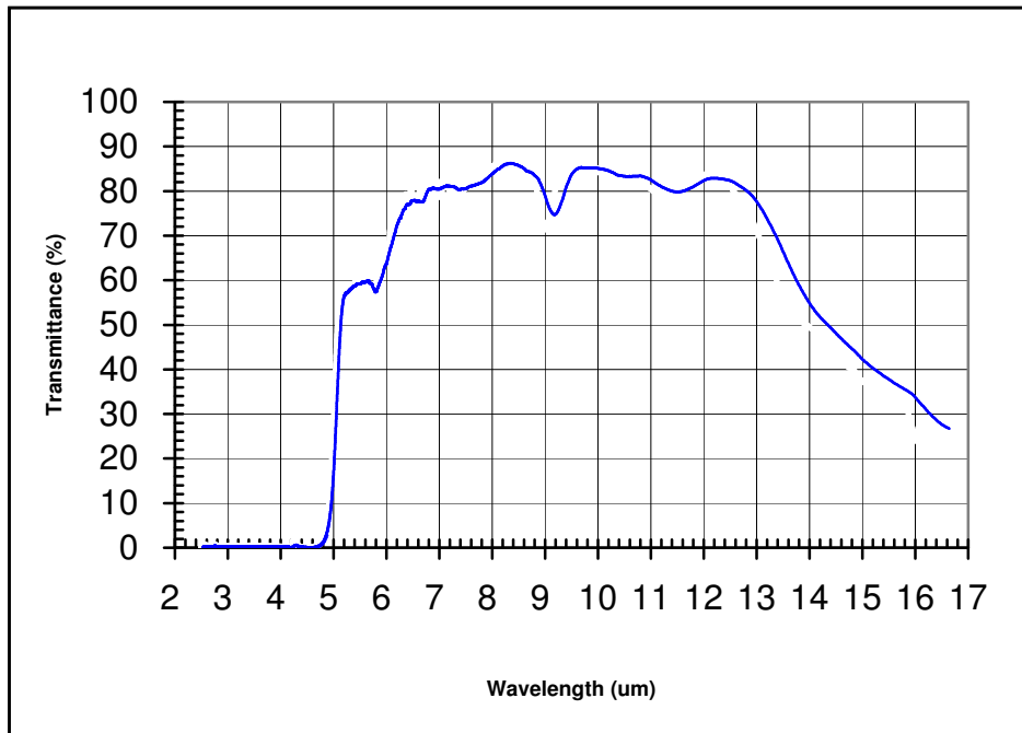
Figure 4: Typical spectral transmittance curve
