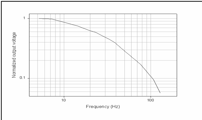
Figure 2: Frequency response
