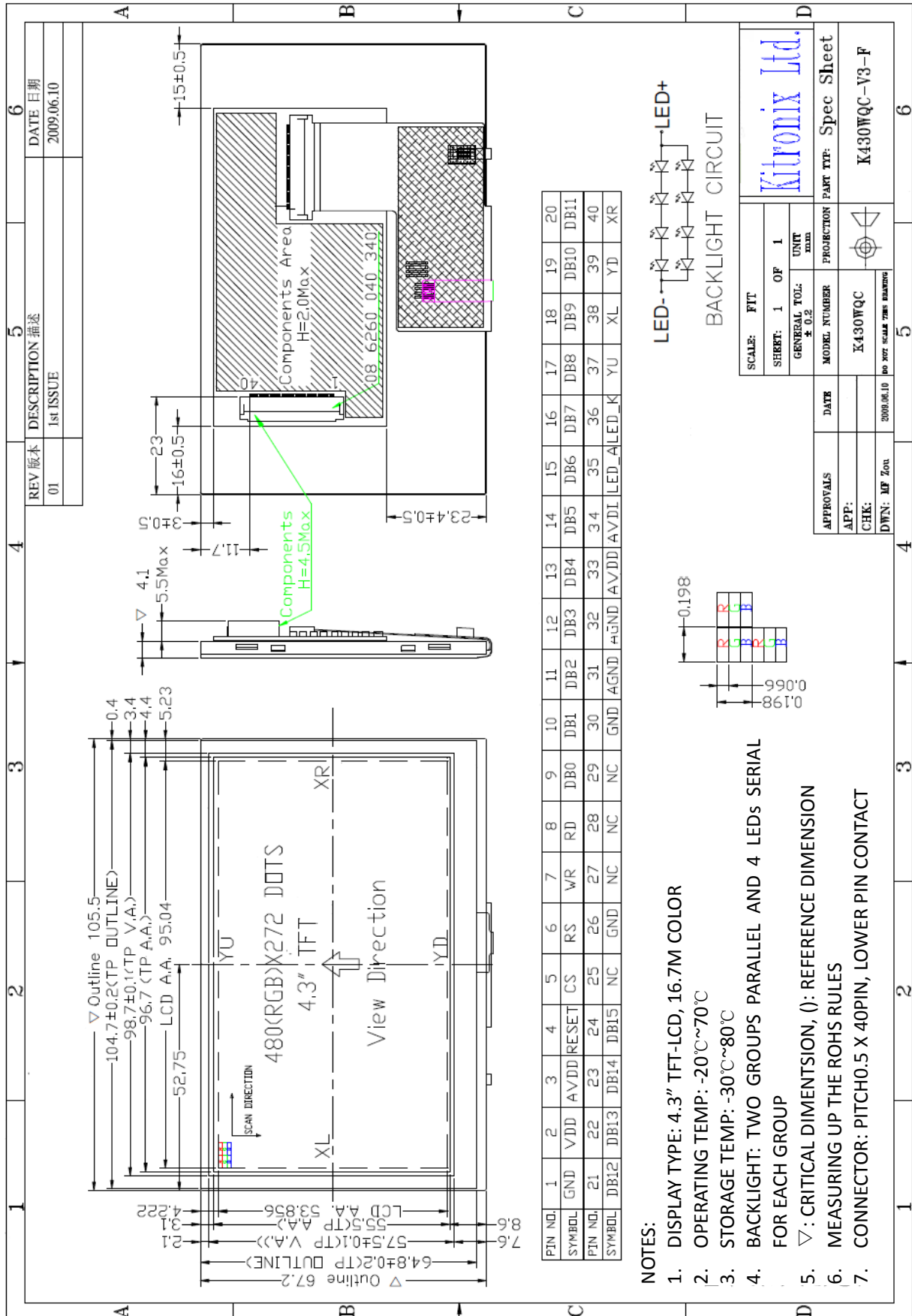
Figure 1: Outline Drawing
