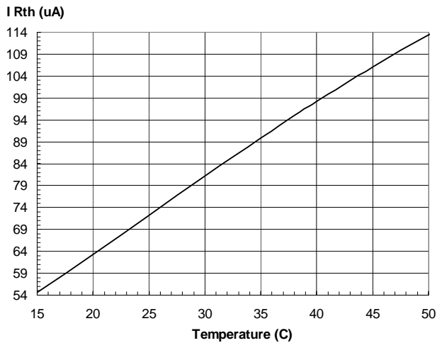
Figure 7. I_{Rth} vs. Temperature
