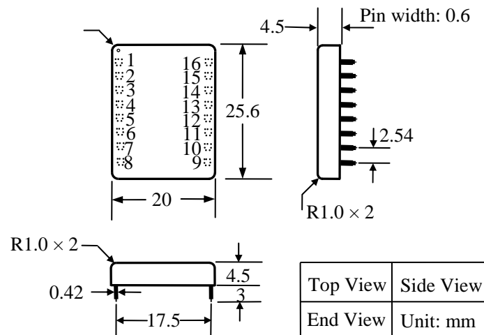
Figure 11. Dimensions of the DIP package controller of TEC6A5V-D
