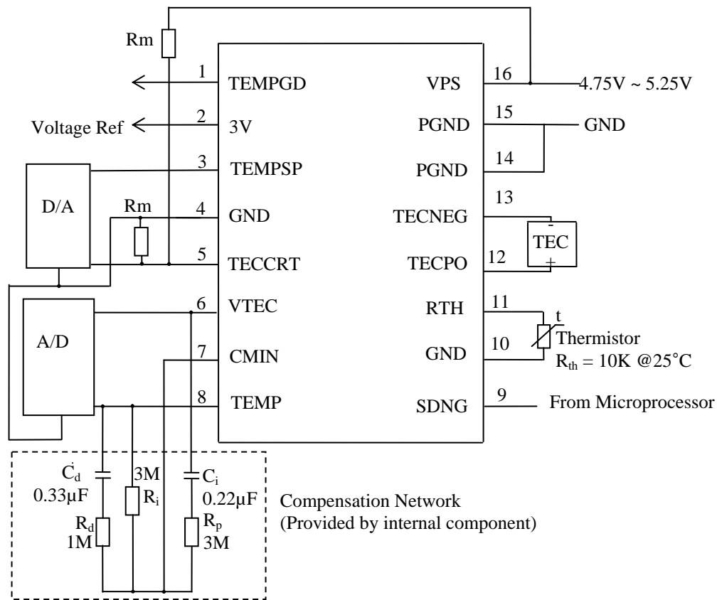
Figure 4. TEC Controller Connections
