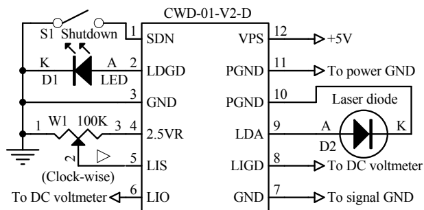
Figure 4 A Typical Stand-alone Application Schematic
