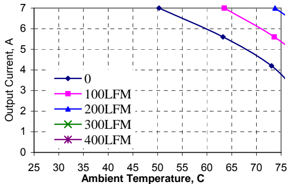
Figure 7. HLD15ZGE Derating Curves
