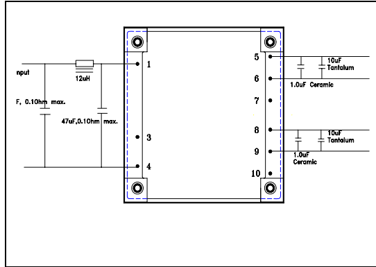
Figure 5. Typical Application of HLD Series
