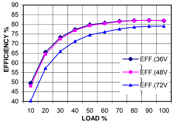
Figure 4. HLD15ZEB Efficiency vs. Output Load
