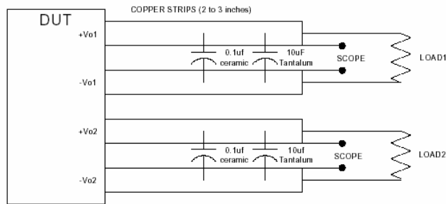
Figure 6. . Output Ripple & Noise Measurement Test Setup
