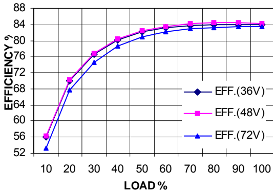
Figure 2. HLD15ZED Efficiency vs. Output Load
