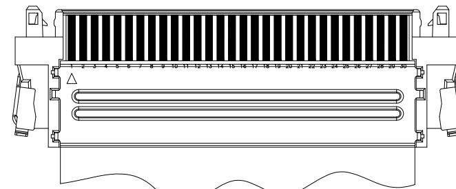
Mated condition (REF.)
