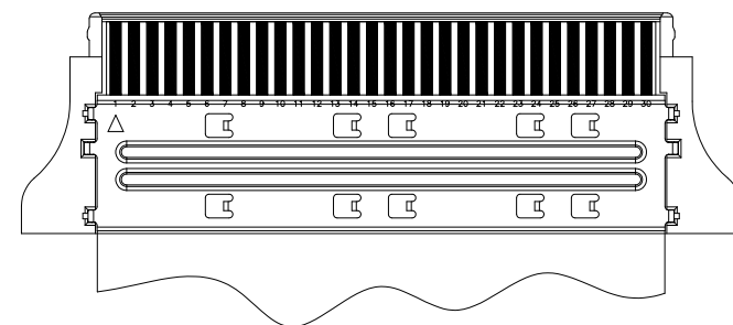
Mated condition (REF.) A1001FH-30P + A1001F-B
