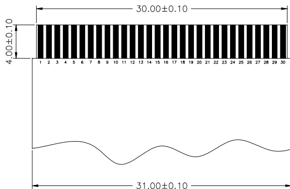
Recommended FFC dimension
