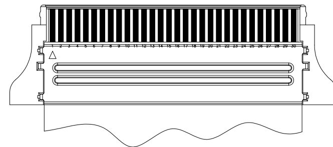
Mated condition (REF.) A1001FH-30P + A1001F-A
