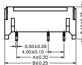
A4001WR-S-4P-157
