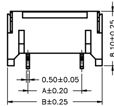
A4001WR-S-2P-2
