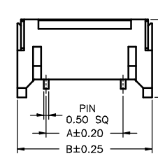
A4001WR-2P-2
