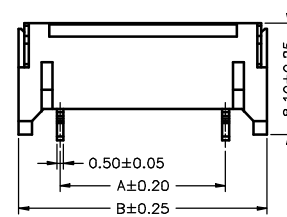
A4001WR-S-2P-3
