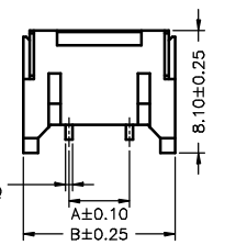
A4001WR-2P-1
