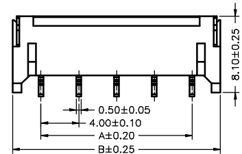
A4001WR-S-5P
