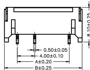
A4001WR-S-4P-137
