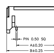
A4001WR-2P-3
