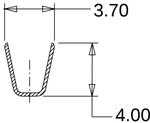
SECTION Y-Y
