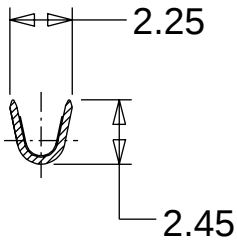
SECTION Z-Z
