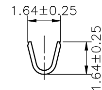
SEC:C-C
