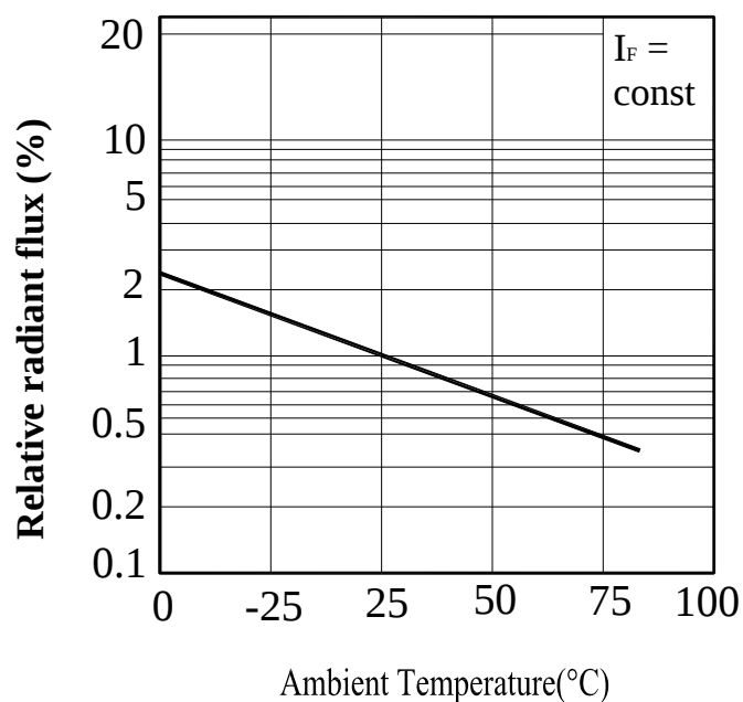
Fig.6 Relative Radiant Flux vs. Ambient Temperature(°C)
