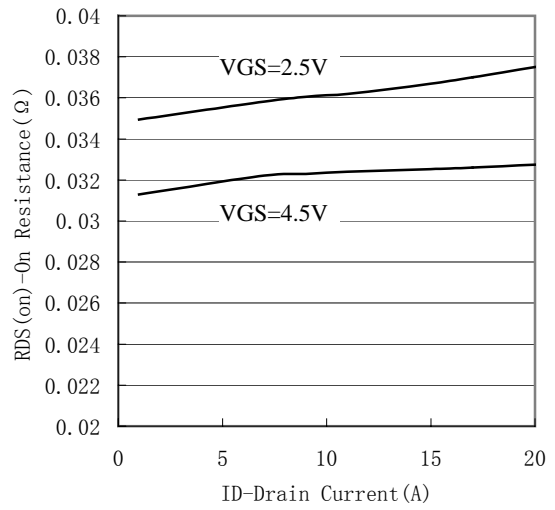
Figure 6. On-Resistance vs. Drain Current
