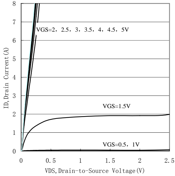
Figure 1. Output Characteristics
