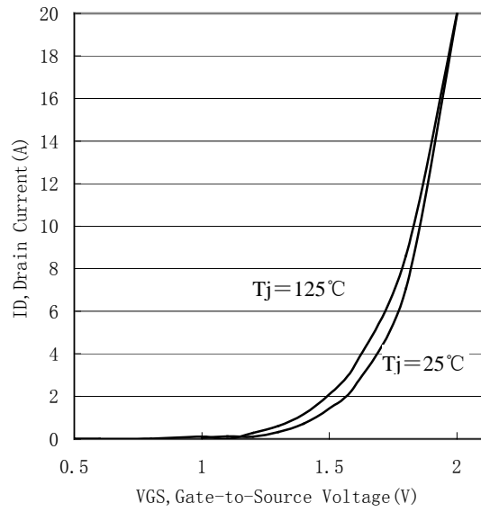
Figure 2. Transfer Characteristics
