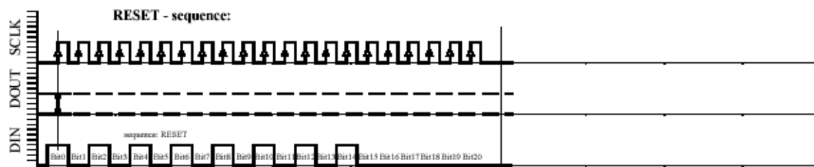
Fig. 6e: Reset sequence (21-Bit)
