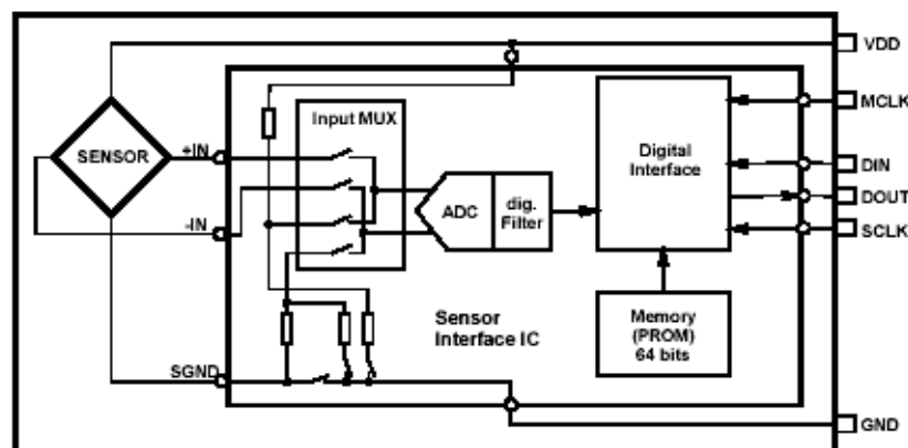
Fig.: 1 Block Diagram 5536
