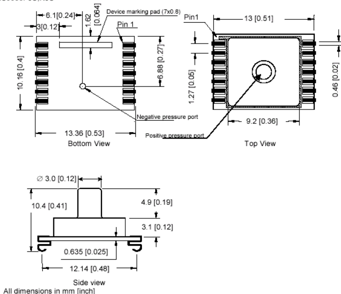
Fig. 8: Device package outlines of MS5536PJU / MS5536NJU
