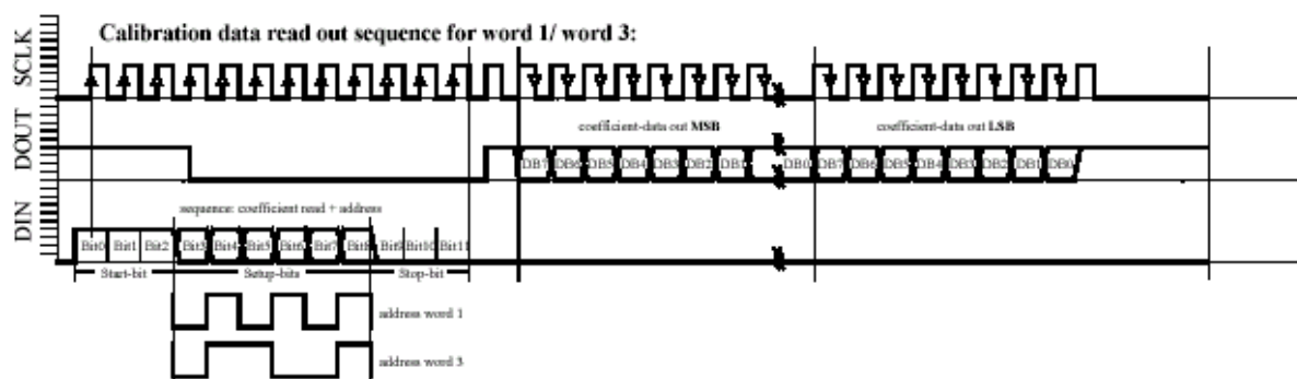
Fig. 6c: W1, W3 reading sequence
