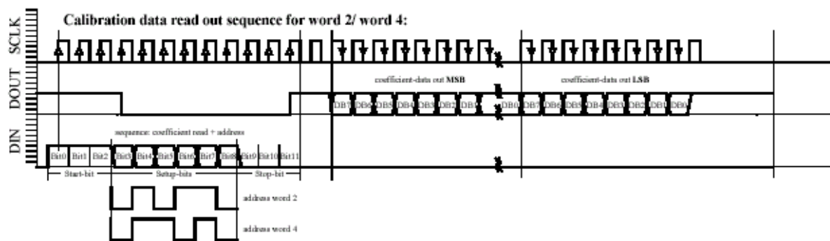
Fig. 6d: W2, W4 reading sequence
