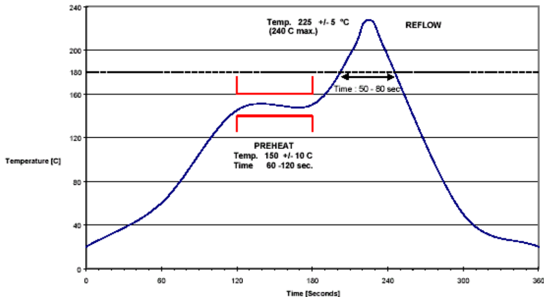
Fig. 10: Recommended soldering profile
