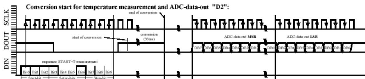
Fig. 6b: D2 acquisition sequence
