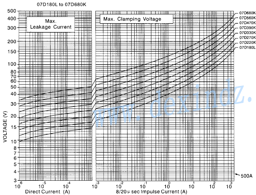
V-I curve
